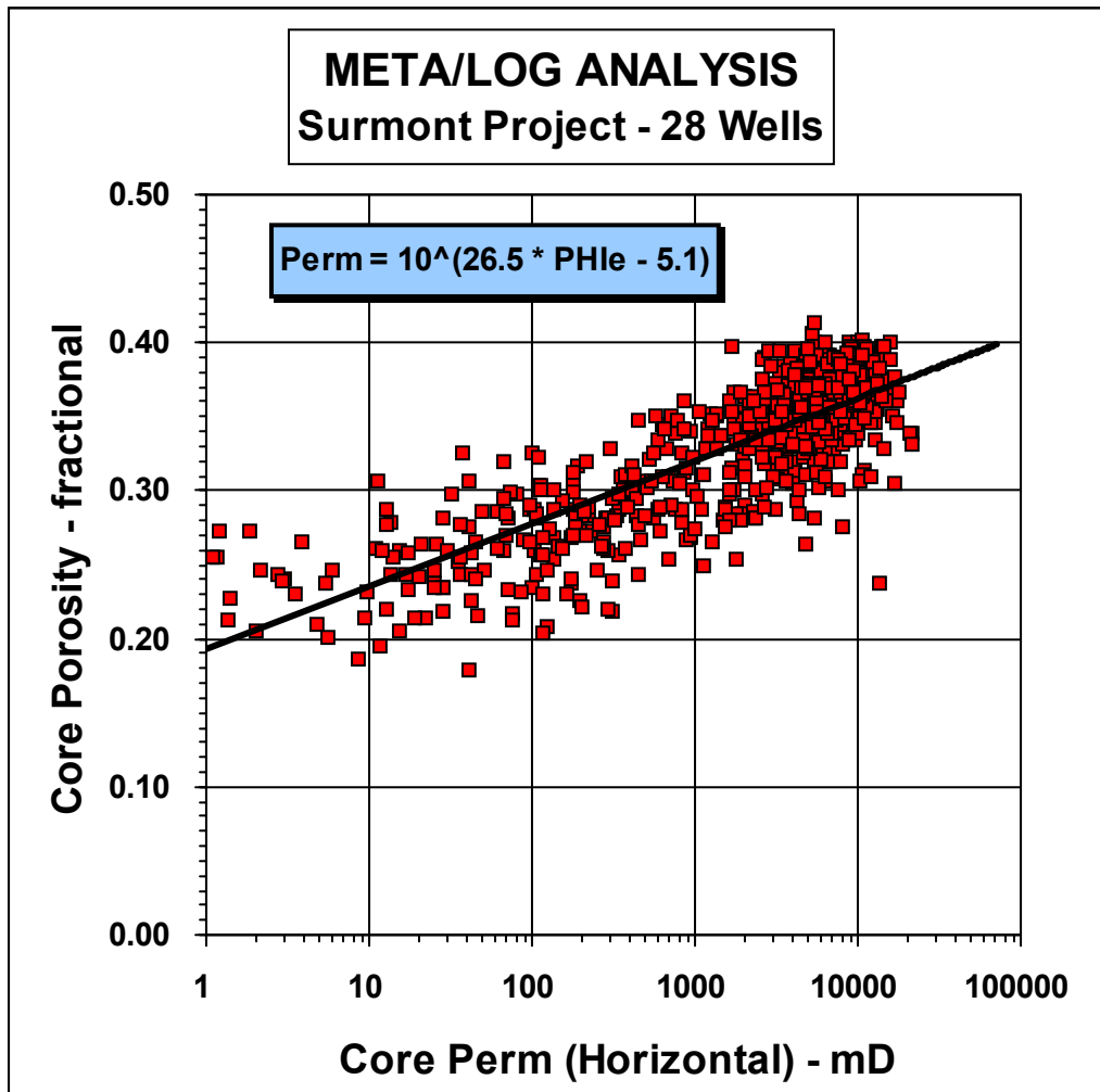
Figure P-1: Core porosity versus permeability under overburden conditions
