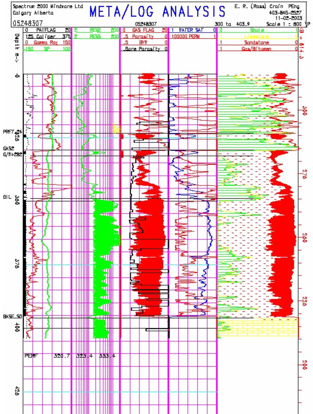
Figure P-4: Results log data for a typical Surmont well
