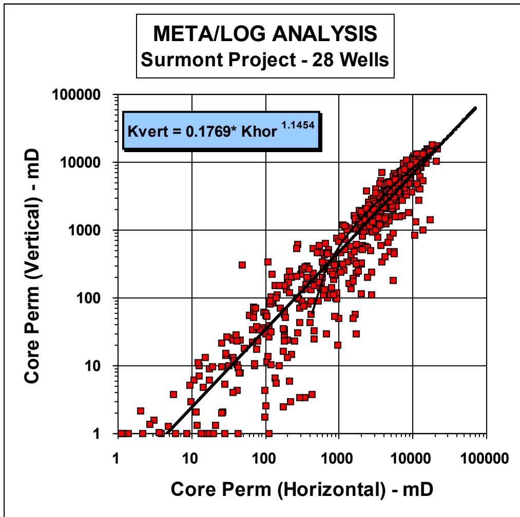
Figure P-2: Vertical versus horizontal permeability under overburden conditions
